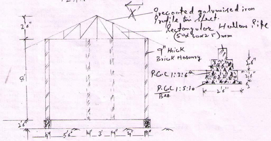
Section X-X
