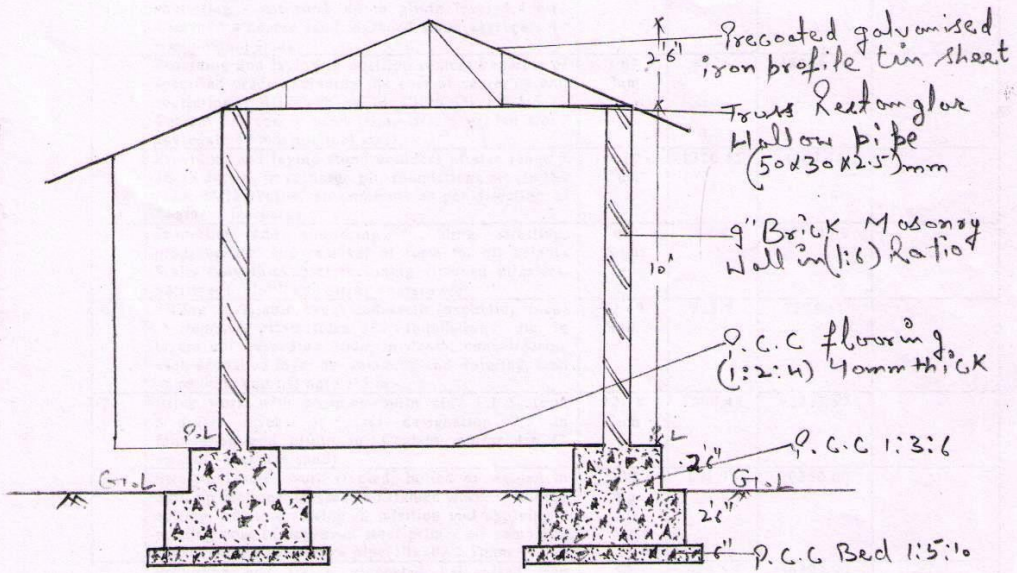
X-Section
